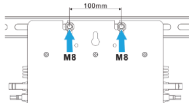
HY-1200-Pro / HY-1300-Pro / HY-2000-Plus
