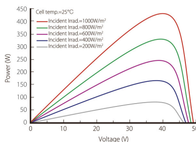
Power-Voltage Curve (LR4-72HPH-430M)
