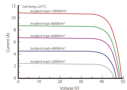
Current-Voltage Curve (LR4-72HPH-430M)
