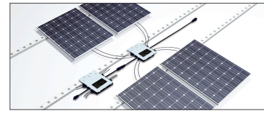
HY-1200-Pro / HY-1300-Pro connected in parallel
